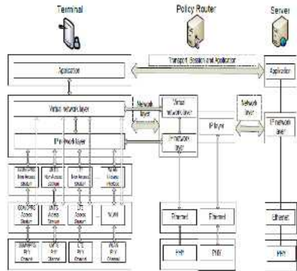
Figure 5: Protocol Layout for the Elements of the Proposed Architecture
