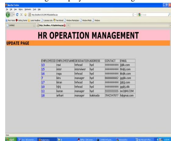
Fig.7 Update Page
