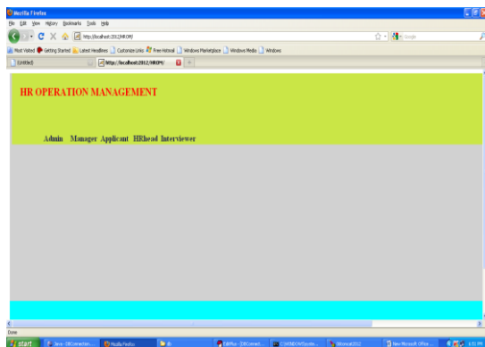
Fig.2 Home page
