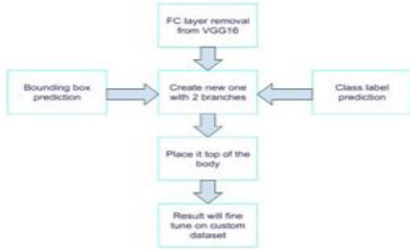
Fig. 2. Creating Network head
