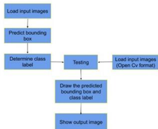
Fig. 7. Testing Flowchart
