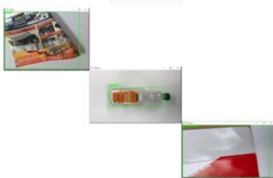
Fig. 8. Detection Output
