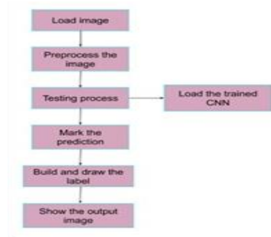
Fig. 11. Classification Testing
