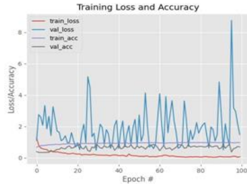
Fig. 10. Training Loss and Accuracy
