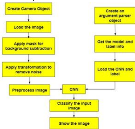
Fig. 13. Web Analysis Flowchart
