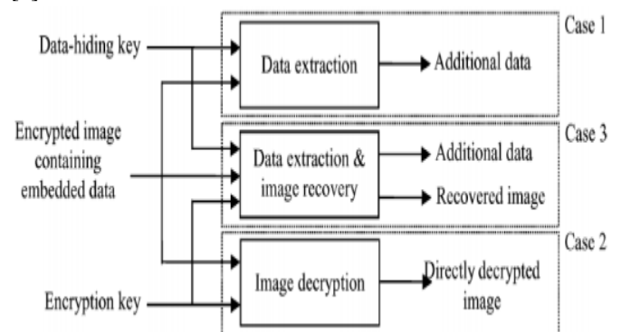
Figure 7. Three cases at receiver side of the proposed separable scheme
