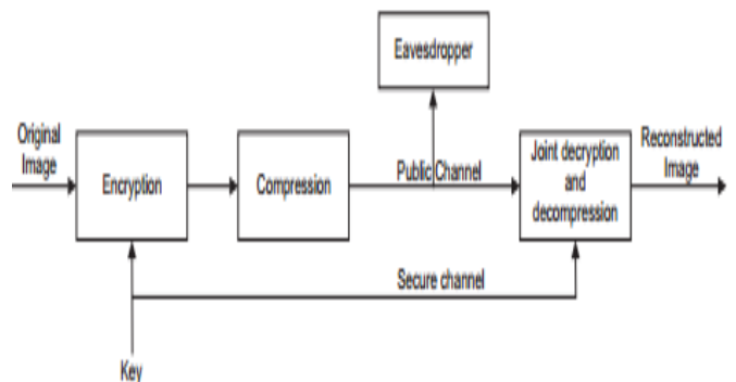
Figure 12: Scheme to compress encrypted images
