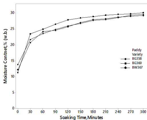
Figure 1: Moisture absorption pattern of BG360, BG358 and BW367 at 70 °C
