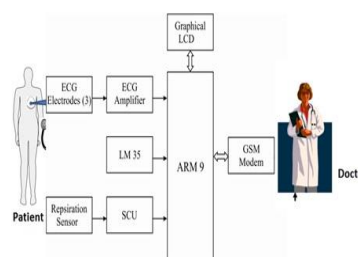
Fig.1: Block diagram of the proposed system
