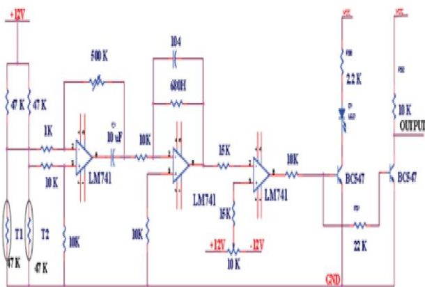
Fig.4: Block Diagram of the Proposed Respiration Circuit
